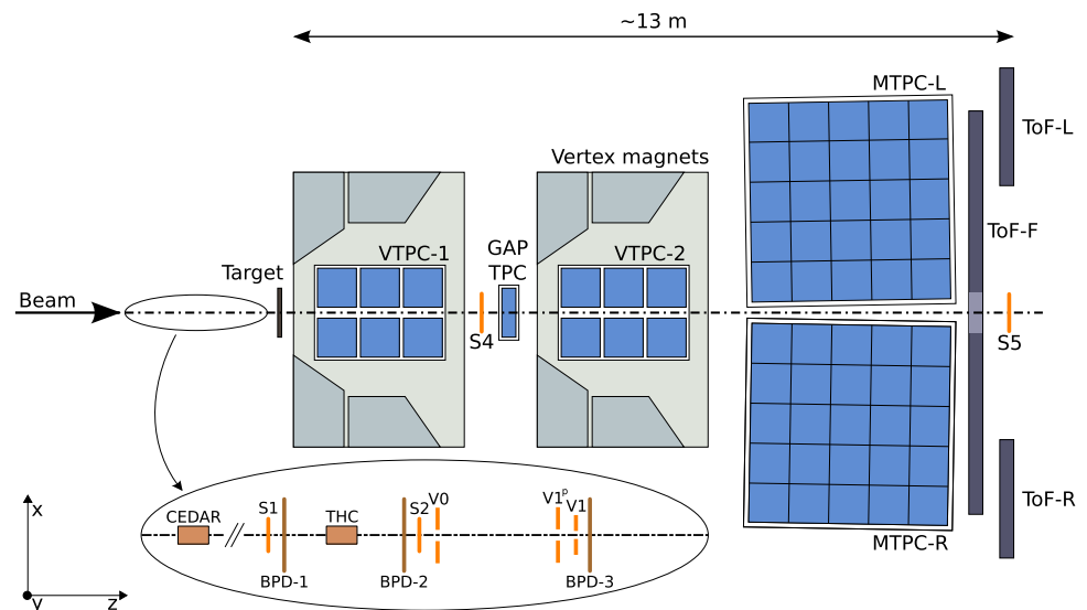
Fig. 1 The schematic layout of the NA61/SHINE spectrometer (horizontal cut, not to scale) used for p+p data taking. The beam and trigger detector configuration is shown in the inset (see Refs. [23, 24] for detailed description). The chosen coordinate system is drawn on the lower left: its origin lies in the middle of the VTPC-2, on the beam axis
