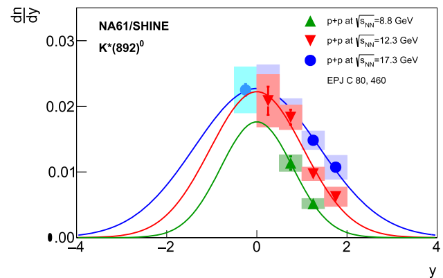
Fig. 8 The rapidity spectra \frac{dn}{dy} of K^*(892)^0 mesons produced in inelastic p+p collisions at 40 GeV/c and 80 GeV/c in transverse momentum range 0 < p_T < 1.5 GeV/c. The numerical values are listed in Table 7. The solid lines represent the function given by Eq. (13). For comparison the previous NA61/SHINE results [9] for p+p interactions at 158 GeV/c are also shown (they were obtained in the full transverse momentum range; p_T -integrated and extrapolated rapidity spectrum). For 158 GeV/c the first (light blue) point ( y < 0 ) was not included in the fit (see Ref. [9] for details)
