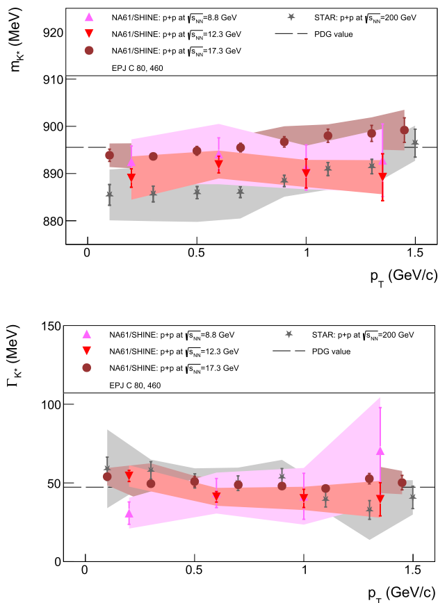
Fig. 10 The transverse momentum dependence of mass and width of K^*(892)^0 (or K^{*0} ) mesons obtained in p+p collisions by NA61/SHINE (this analysis and Ref. [9]) and STAR [11]. For STAR the averaged ( K^{*0} ) measurements of K^*(892)^0 and \bar{K}^*(892)^0 are presented. The horizontal lines represent PDG values [28]
